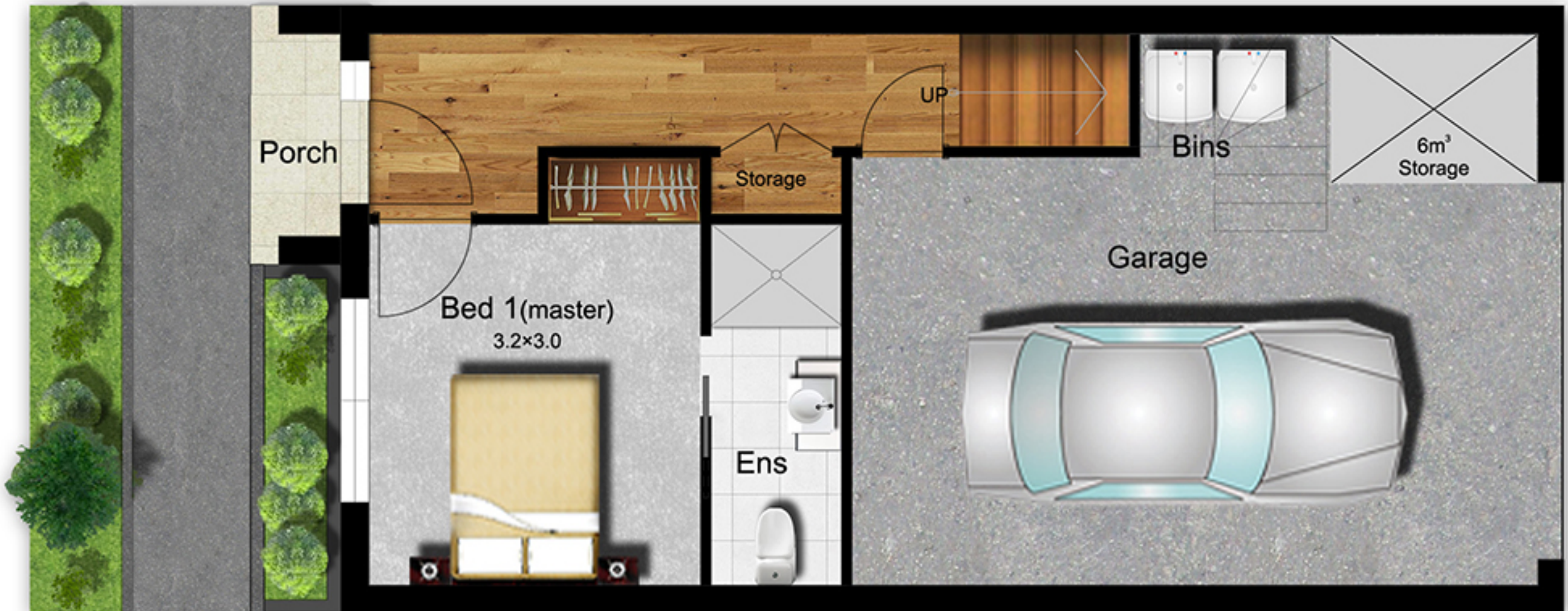
GROUND FLOOR
